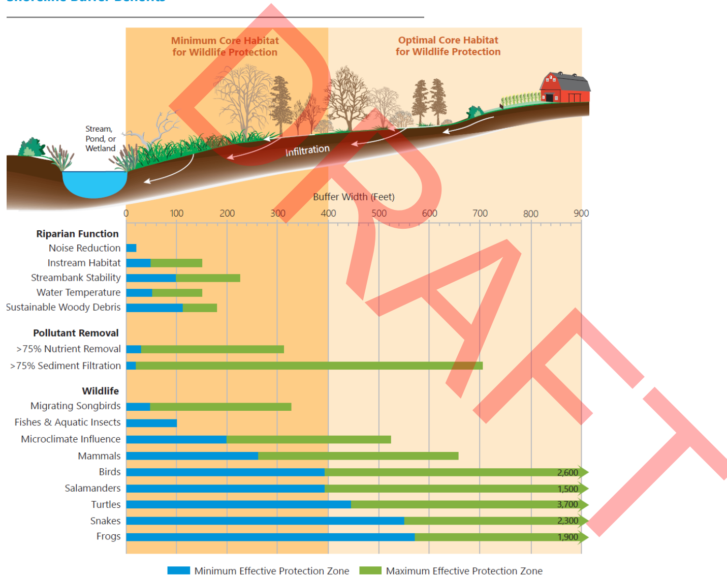
Figure 3.10 Shoreline Buffer Benefits
